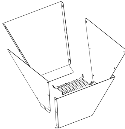
Grain Hopper (4 Pieces) & Finger Protection
